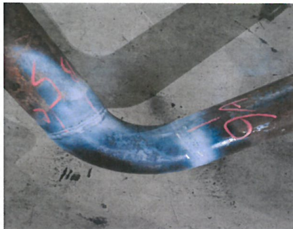
3"-CR-20025-A2-HT45,W5 W6
