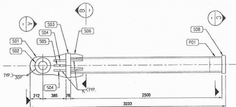
FRONT VIEW Scale: 1/25
